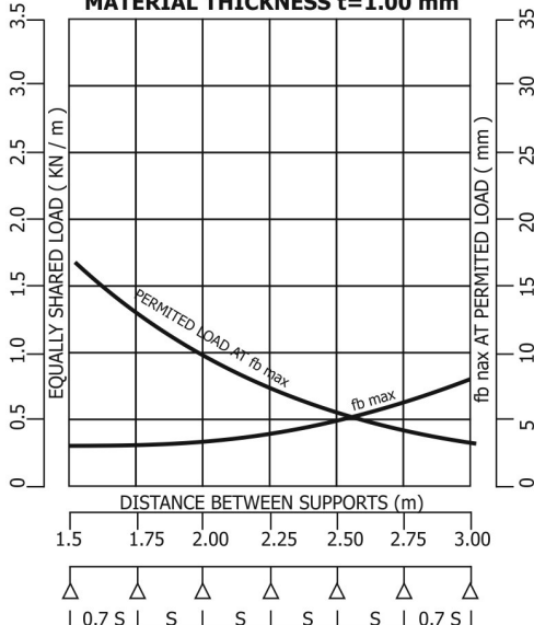
CABLE TRAY H:85 LOADING DIAGRAM
